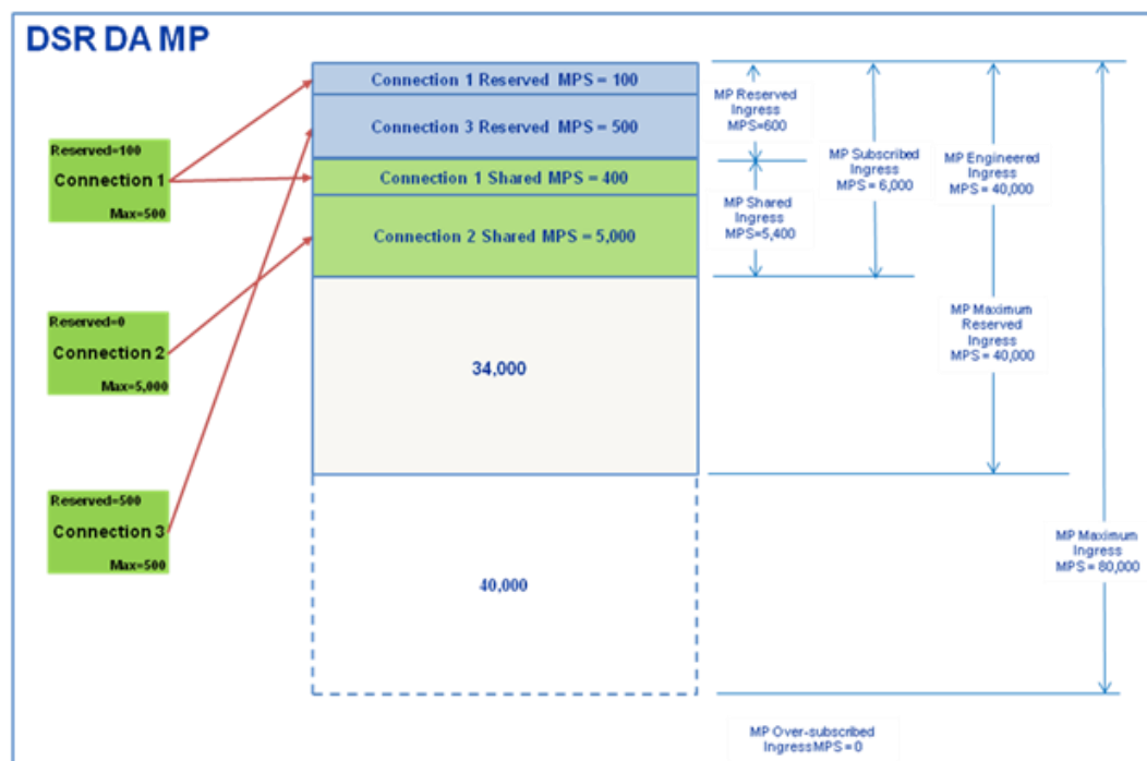
Figure 22 – DSR Ingress MPS Configuration Example 1 – Normal Case
