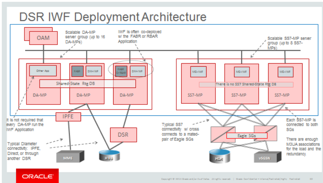
Figure 54 - DSR with MAP-Diameter IWF
