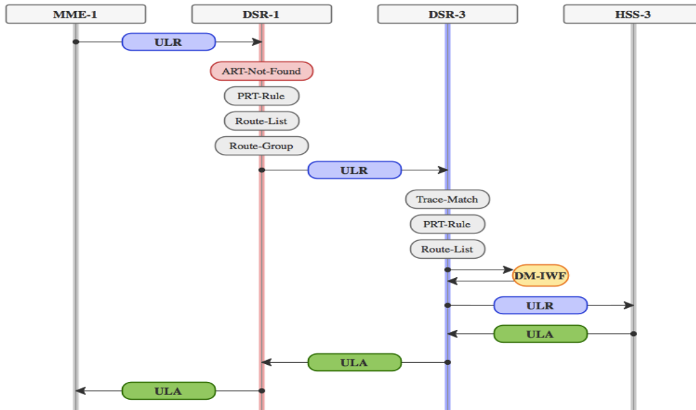
Figure 72 – Message Flow for Network Wide Trace
