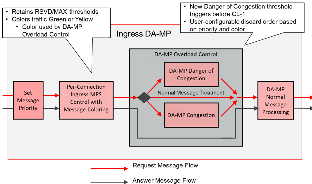
Figure 23 – Message Coloring and Priority/Color-based DA-MP Overload Control
