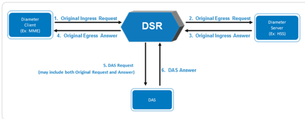
Figure 67 - Message Copy Overview
