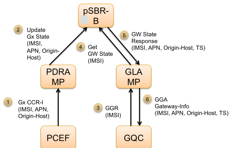
Figure 63 - IMSI Query with Single Matching Gx Session Use Case
