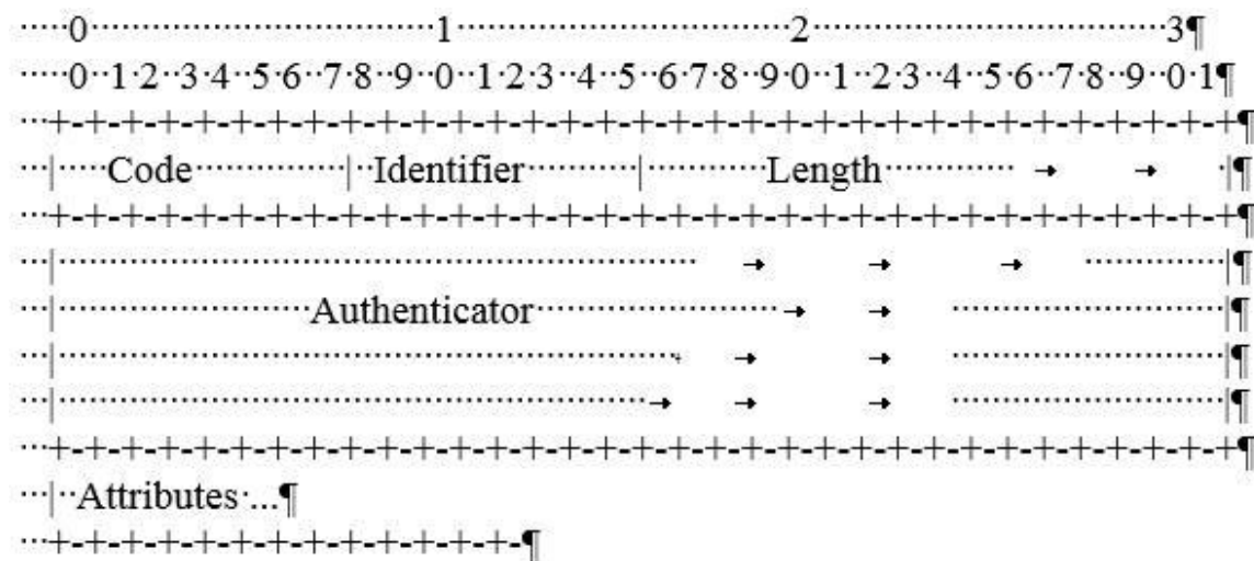
Figure 44 – RADIUS Data Format
