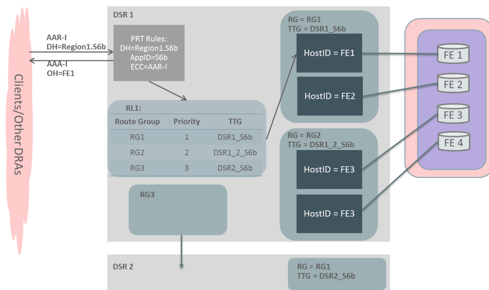
Figure 38 - Congestion-Aware Route List Example 1
