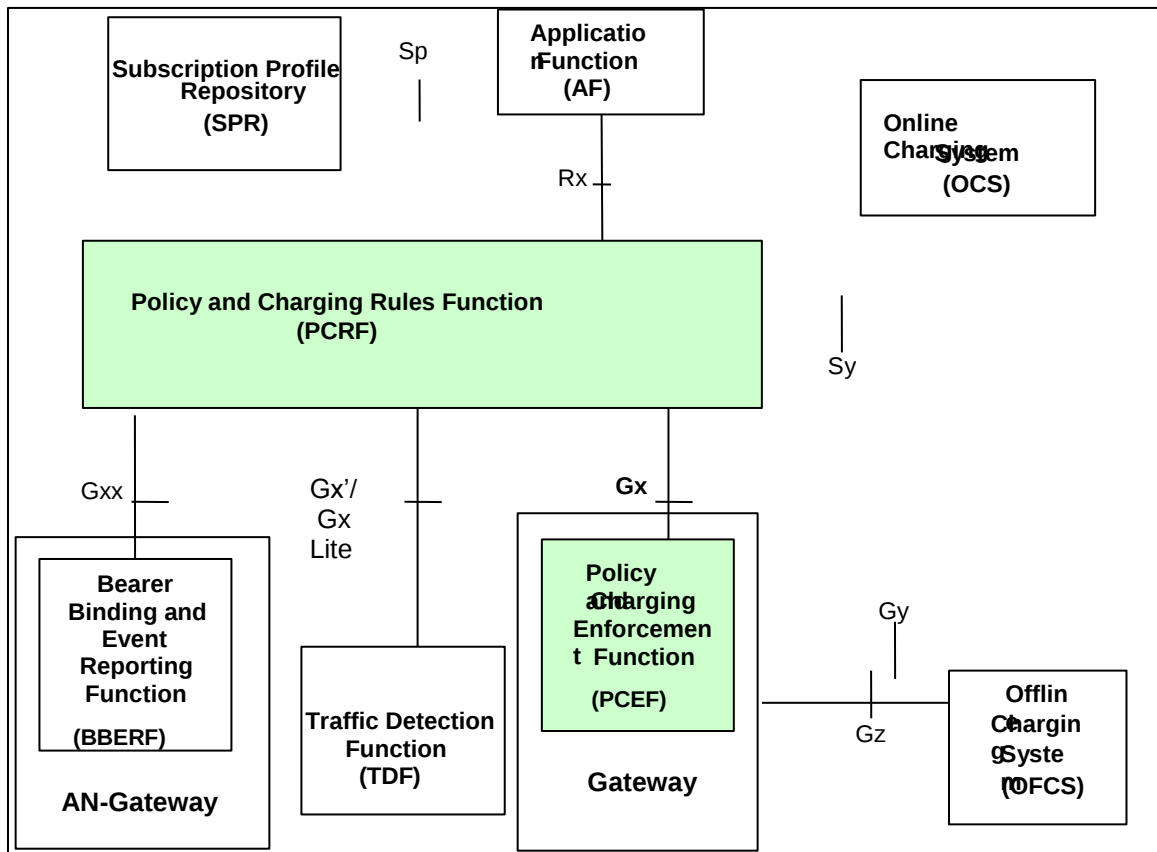
Figure 58 - Overall PCC logical architecture (non-roaming)
