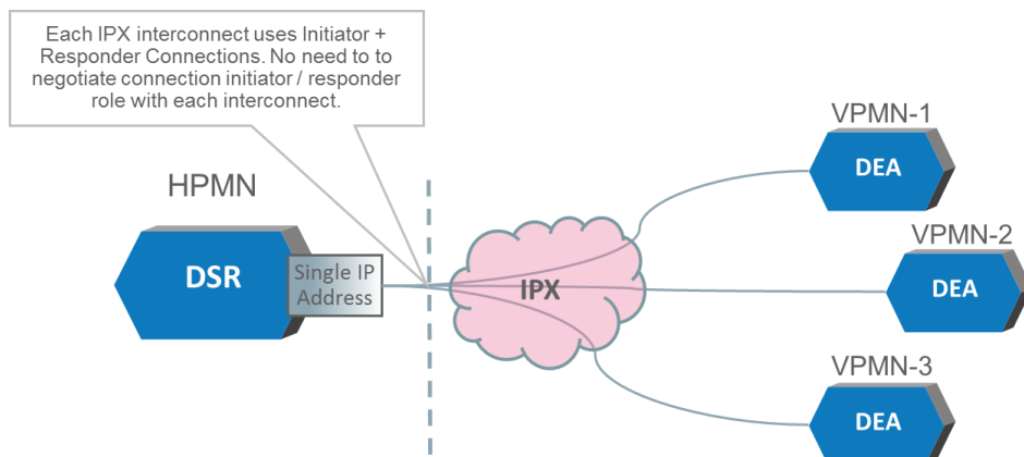
Figure 42 - IPFE Initiator + Responder Support
