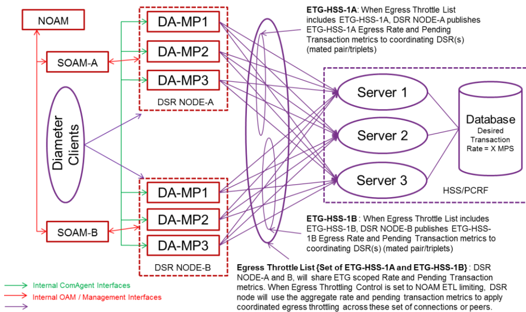
Figure 27 – 2 DSR Sites: Coordinated Egress Throttling Example
