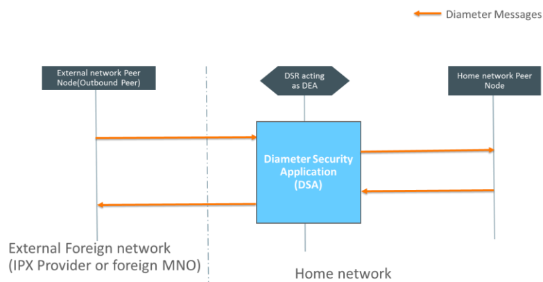
Figure 66 – Diameter Security Application (DSA)
