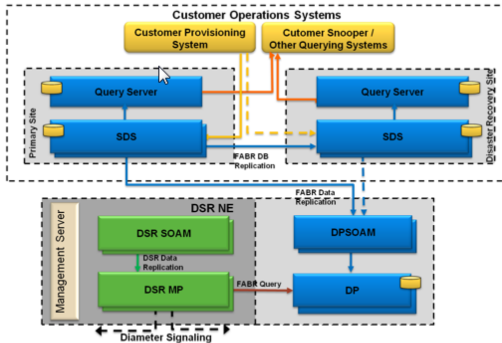
Figure 53 - Subscriber Data Server Architecture
