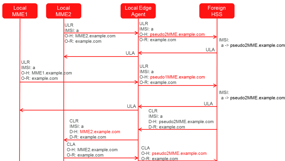
Figure 49 - MME/SGSN Topology Hiding
