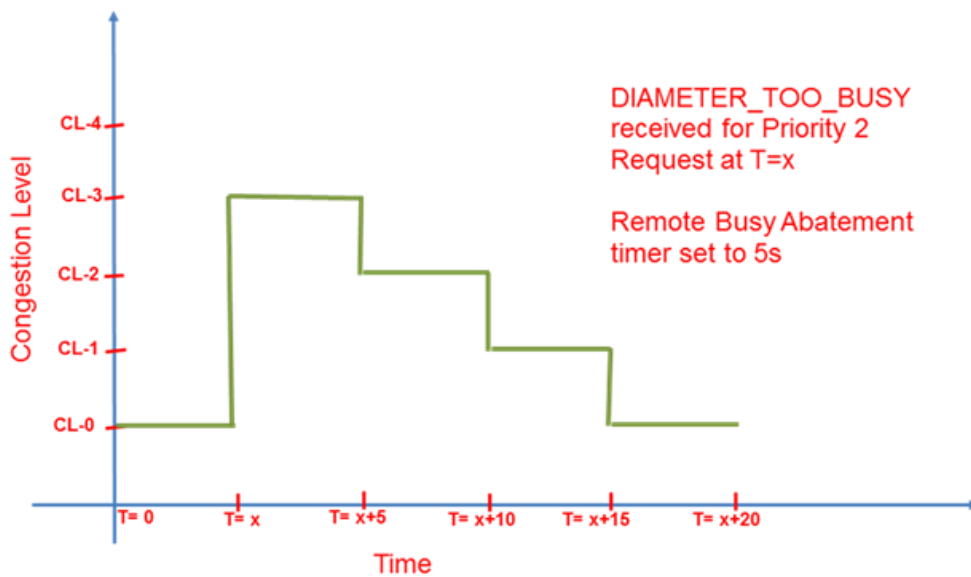
Figure 29 – Congestion level abatement over time for Remote Busy
