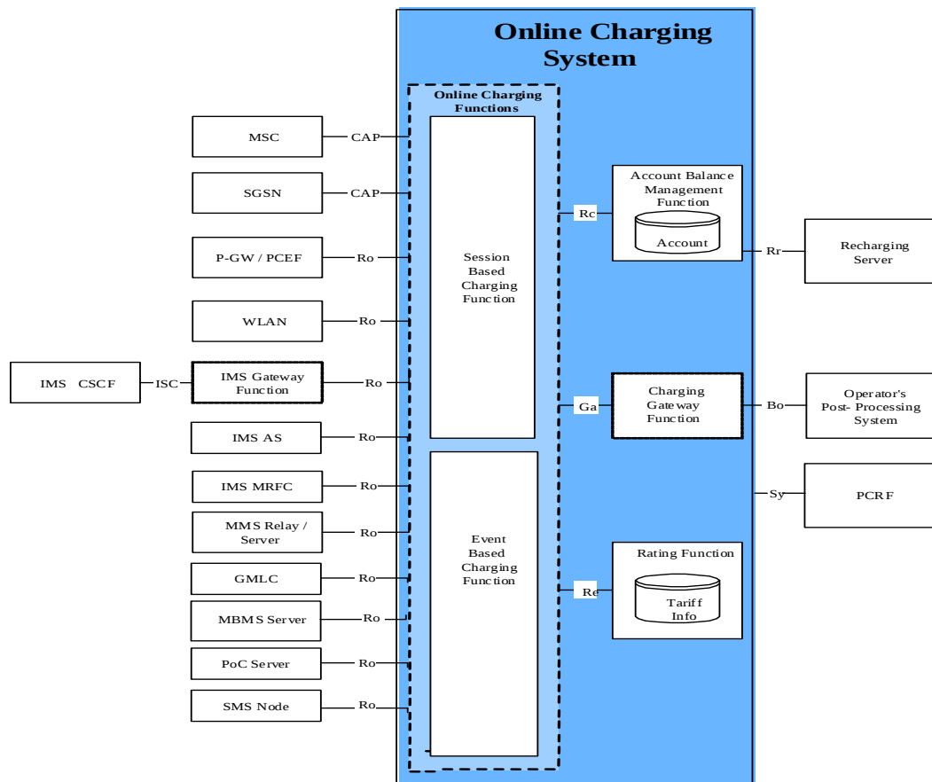
Figure 55 - Online Charging System and Architecture
