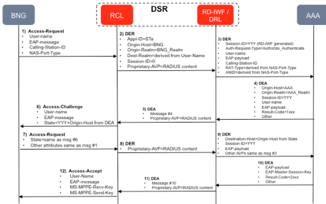
Figure 47 - RADIUS->Diameter IWF for Authentication
