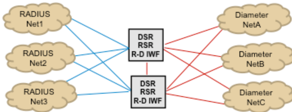
Figure 46 - RSR and R-D IWF Deployment
