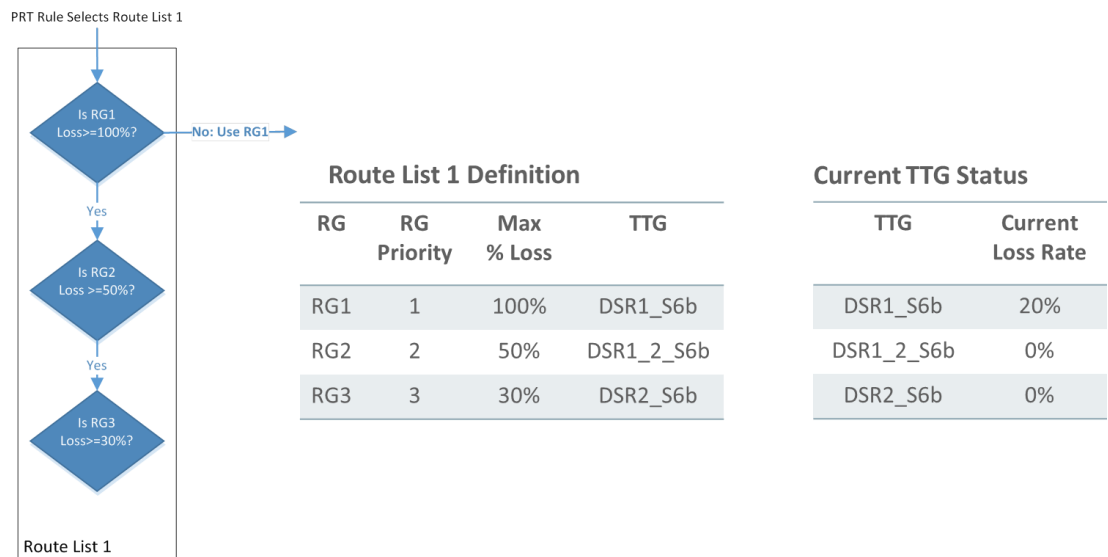
Figure 37 - Congestion-Aware Route List Logic
