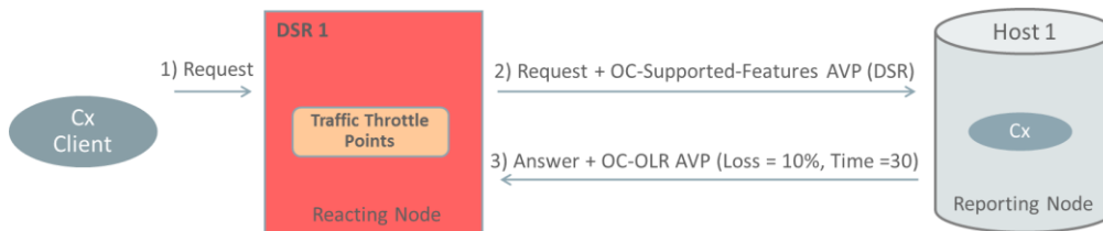
Figure 32 – DOIC Overload Reports Example
