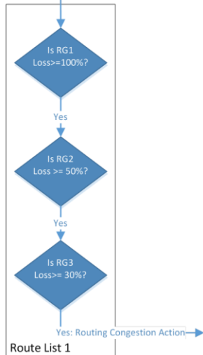
Figure 40 - Congestion-Aware Route List Logic Example 1b
