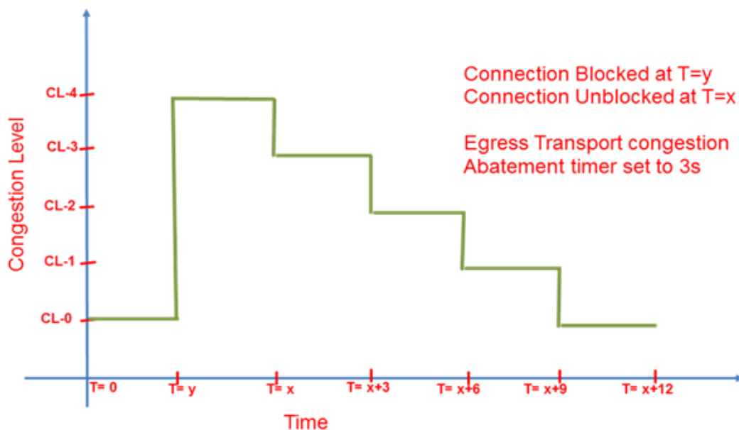
Figure 24 – Example Congestion level abatement
