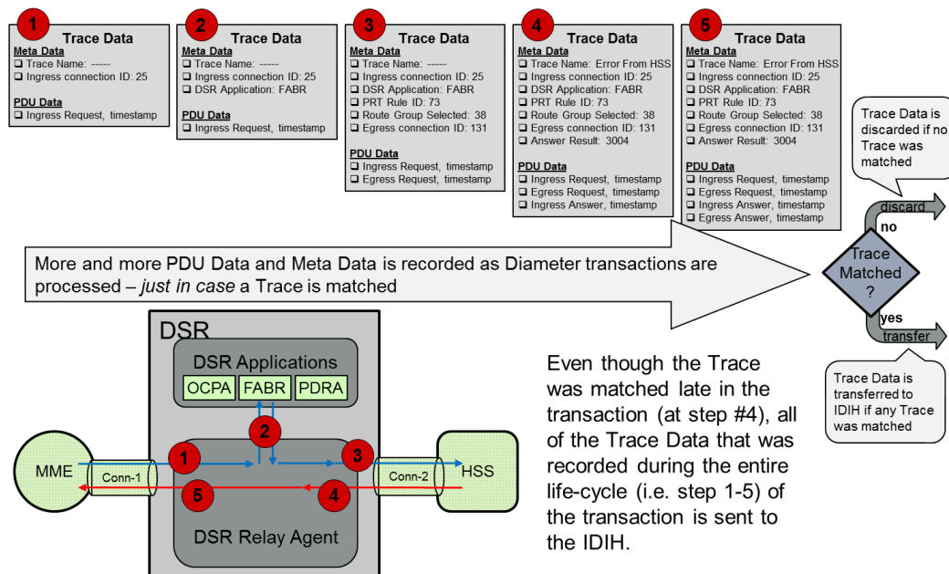
Figure 70 - IDIH Trace Data
