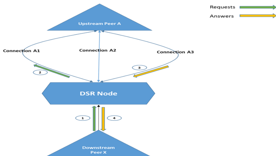
Figure 20 - Answer processing on connection different from the connection used to send Request message
