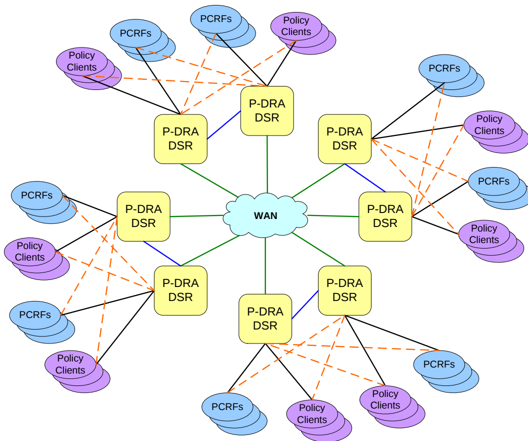
Figure 57 – Network View of P-DRA Mated Pairs
