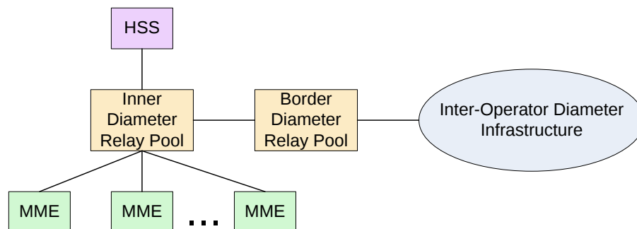
Figure 2 - 3GPP Inter/Intra-operator Diameter infrastructure
