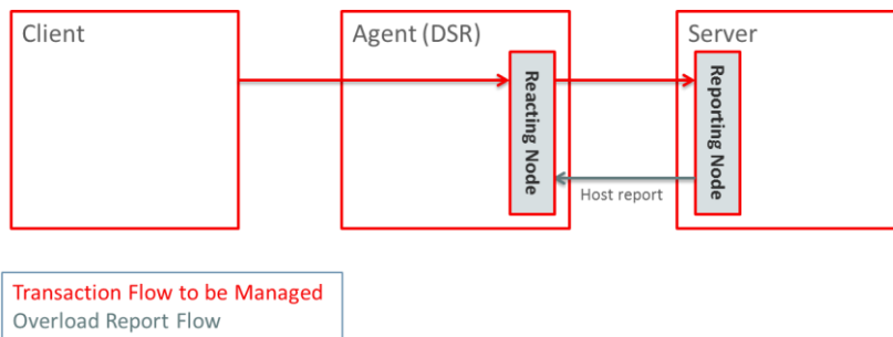
Figure 30 - Reacting Node Role for DOIC
