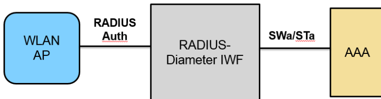
Figure 45 - RADIUS-Diameter IWF for WLAN Authentication
