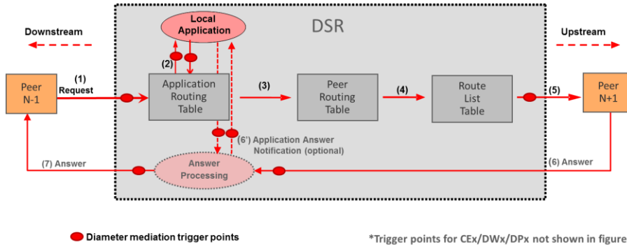
Figure 48 - Mediation Trigger Points
