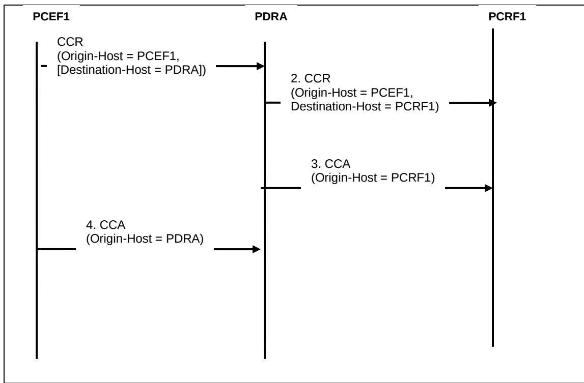
Figure 59 - PCRF topology hiding
